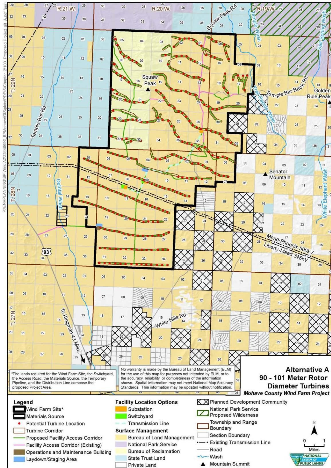
Figure 1-3: Site Layout for Wind Turbines
