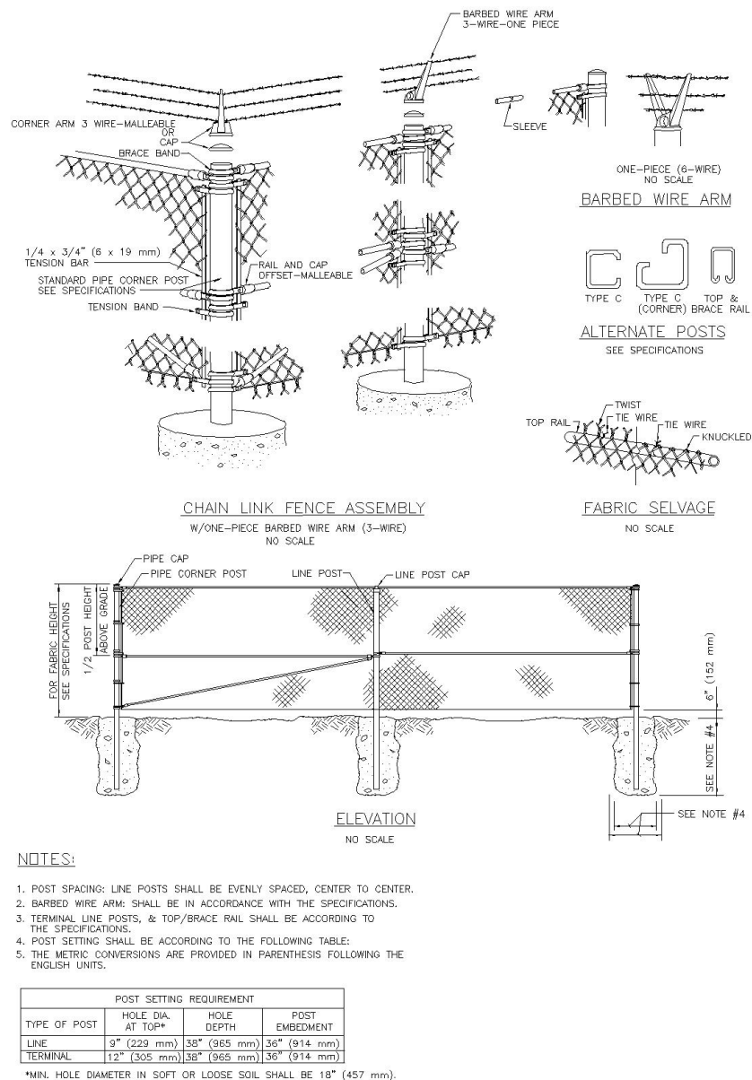
Figure 1-4: Fencing Diagram
