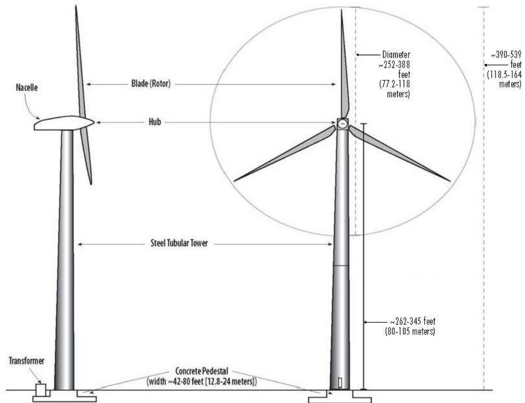
Figure 1-2: Wind Turbine Schematic
