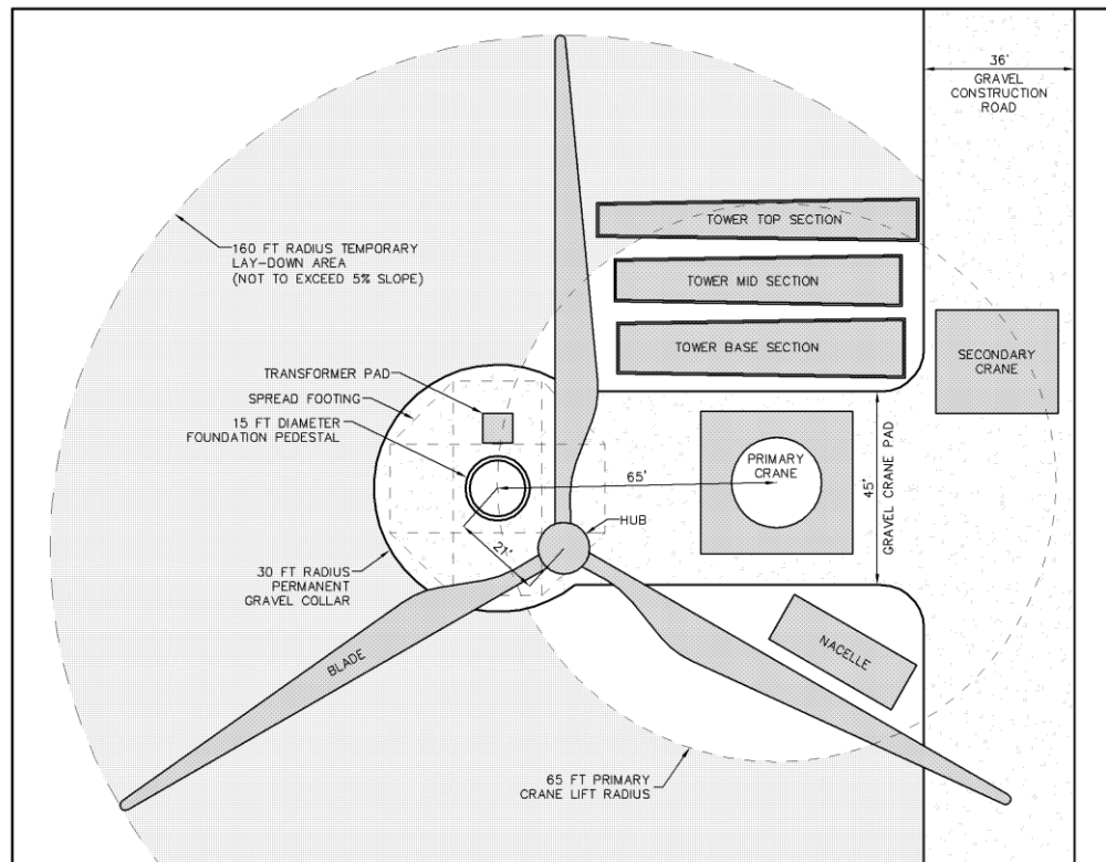
Figure 2-6: Wind Turbine Generator Component Staging and Assembly
