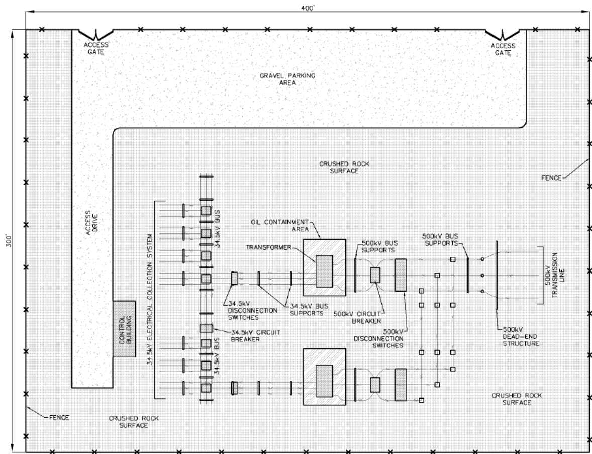
Figure 2-10: Typical Substation Facility Layout
